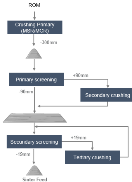
Figure 14-1: Simplified flowsheet.
