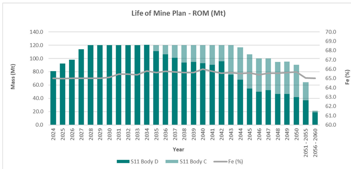
Figure 13-7: Life of Mine vs Fe grades.
