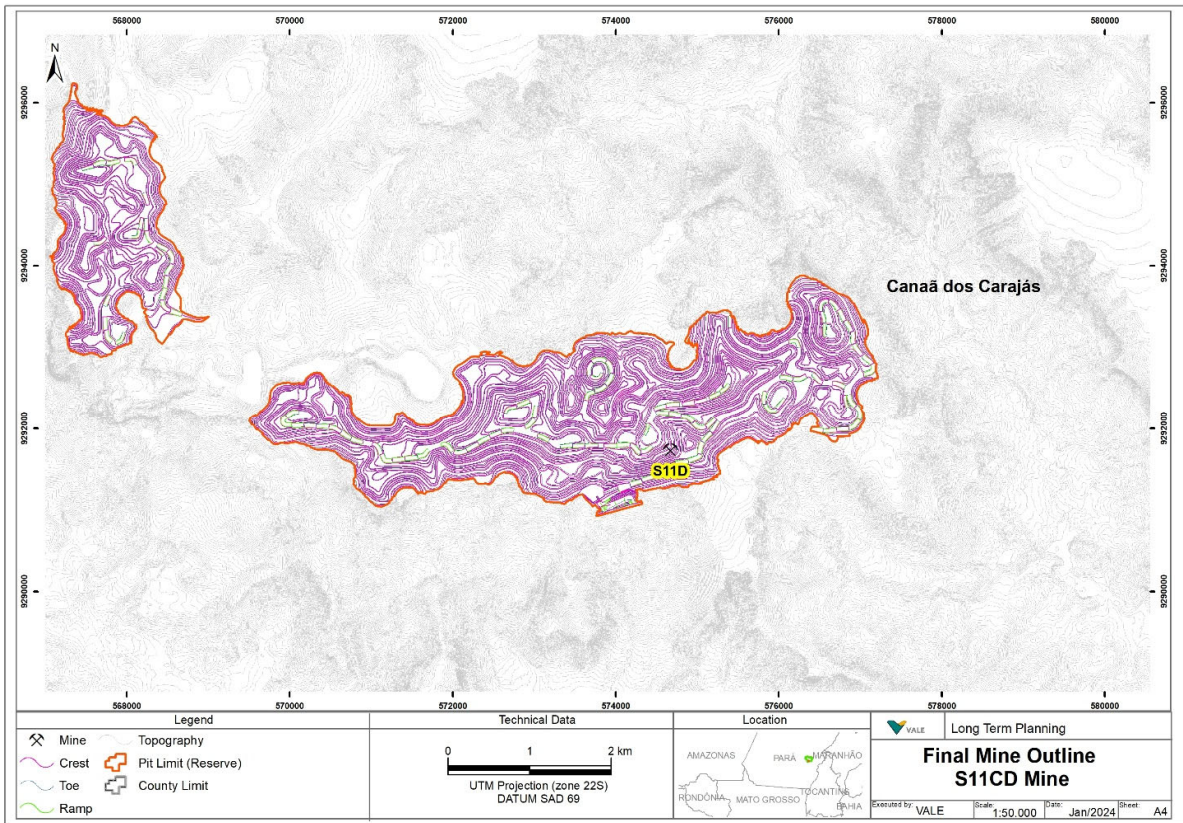
Figure 13-1: Open-pit design.
