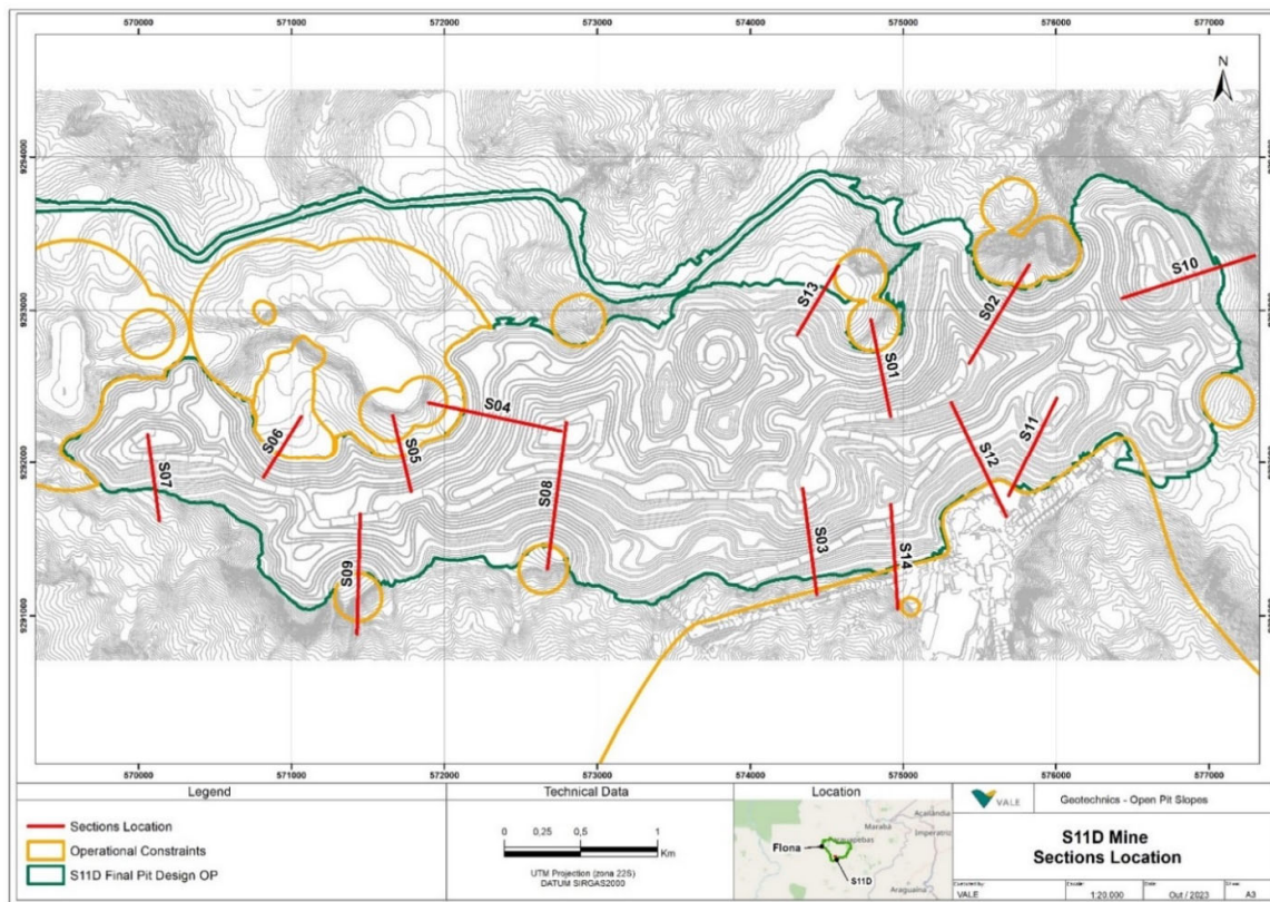
Figure 13-4 - Slope stability analysis cross-section location – S11D mine
