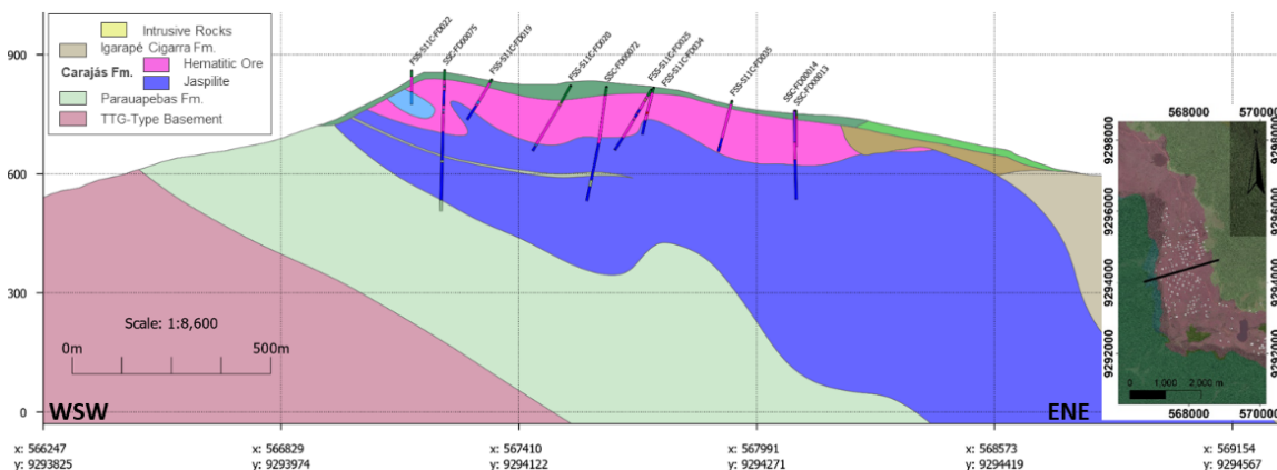
Figure 6-8 – Geological section of SSC.
