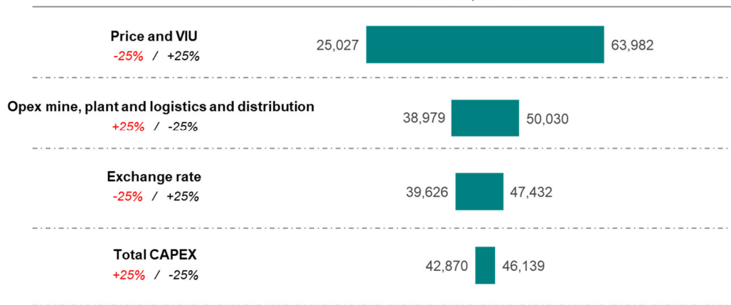
Figure 19-2- Sensitivity Analysis
