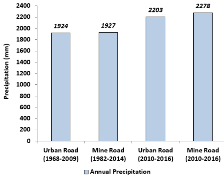
Figure 17-1: Serra Sul historical annual precipitation.
