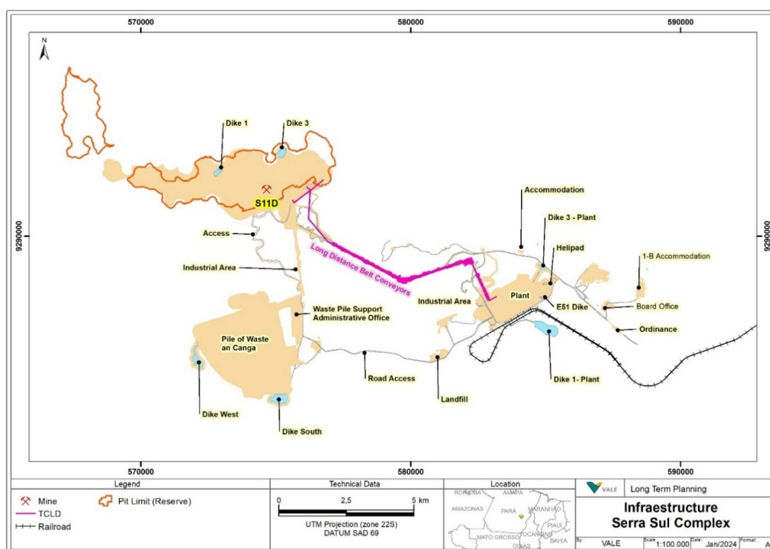
Figure 15-1: Mine site infrastructure map
