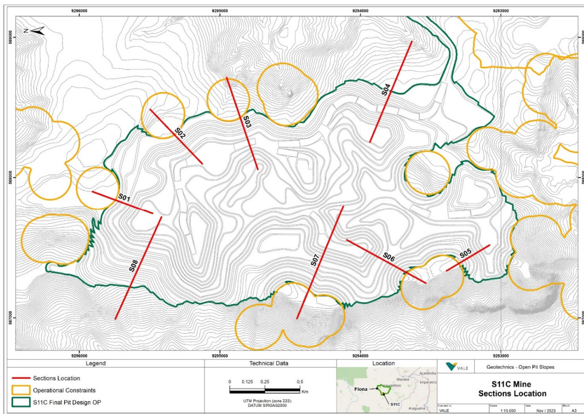
Figure 13-3 - Slope stability analysis cross-section location – S11C mine.
