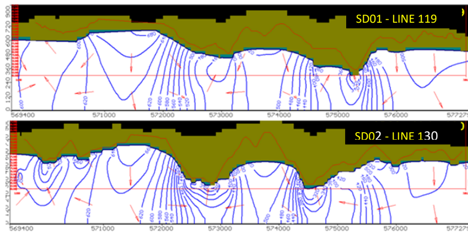
Figure 13-6 Maximum drawdown cross sections
